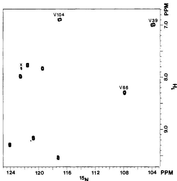
FIGURE 4: ^1\text{H} - ^{15}\text{N} HMQC spectrum of Nase labeled with [1-^{13}\text{C}]\text{-L}/[^{15}\text{N}]\text{V} . One Val signal at \delta_{\text{H}}, \delta_{\text{N}} 10.18, 136.1 lies outside the portion of the spectrum shown. The weak signal indicated by the x has not been identified.
