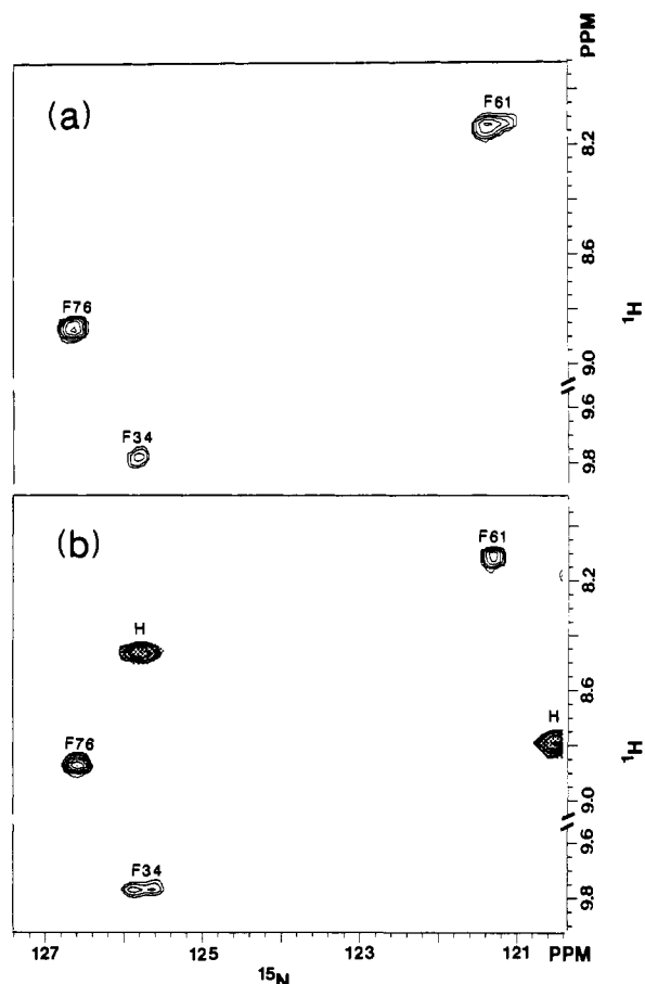
FIGURE 2: Comparison of ^1\text{H} - ^{15}\text{N} HMQC spectra of Nase labeled with (a) [1\text{-}^{13}\text{C}]\text{A}/[^{15}\text{N}]\text{F} and (b) [1\text{-}^{13}\text{C}]\text{T}/[^{15}\text{N}]\text{F}/[^{15}\text{N}]\text{H} . The signal assignments given in these and subsequent spectra are discussed in the text. The shaded signals in (b) are due to His residues.
