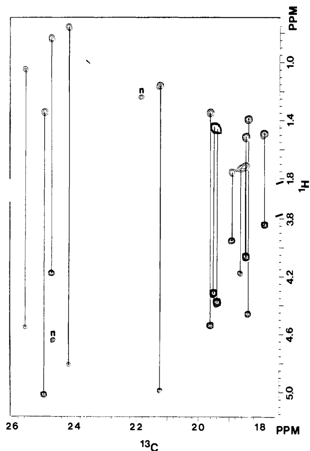
FIGURE 6: HMQC RELAY spectrum of Nase labeled with [3\text{-}^{13}\text{C}]\text{A} , showing the correlated \alpha -proton and methyl proton signals of each of the 14 Ala residues in Nase. The weak uncorrelated signals, labeled n, are due to protons bonded to ^{13}\text{C} nuclei in natural abundance. Note the break in the proton chemical shift axis.
