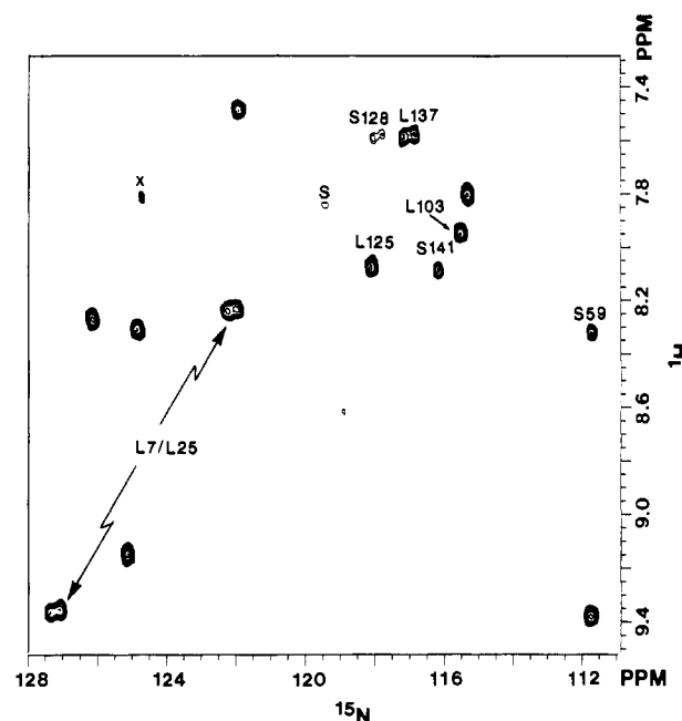
FIGURE 5: ^1\text{H} - ^{15}\text{N} HMQC spectrum of Nase labeled with [1-^{13}\text{C}]\text{-K}/[^{15}\text{N}]\text{L}/[^{15}\text{N}]\text{S} . The Leu and Ser signals were identified in spectra of Nase samples which contained either [^{15}\text{N}]\text{L} or [1-^{13}\text{C}]\text{W}/[^{15}\text{N}]\text{S} . The spectrum of the latter sample (not shown) shows a split signal at \delta_{\text{H}} 8.09 which is assigned to S141 because W140 is the only Trp in Nase. The Leu signals are significantly more intense than the Ser signals because labeled Leu incorporates into Nase with greater efficiency than labeled Ser. The weak signal indicated by the x has not been identified.
